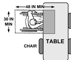
MINIMUM CLEAR FLOOR SPACE SEATING AND TABLES
